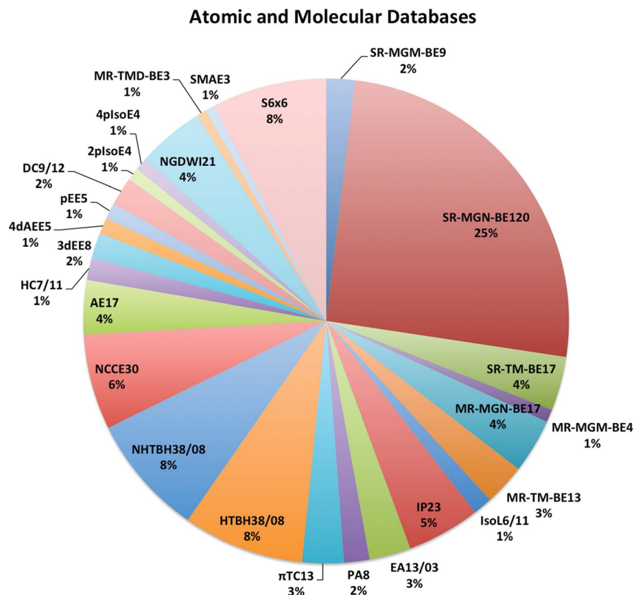
Fig. 1 The percentage of all atomic and molecular databases (AME471), the number after a name means the number of data in this database, for example, SR-MGM-BE9 mean 9 pieces of bonding energy data in this database. The explanation of these names are shown in Table 1.
