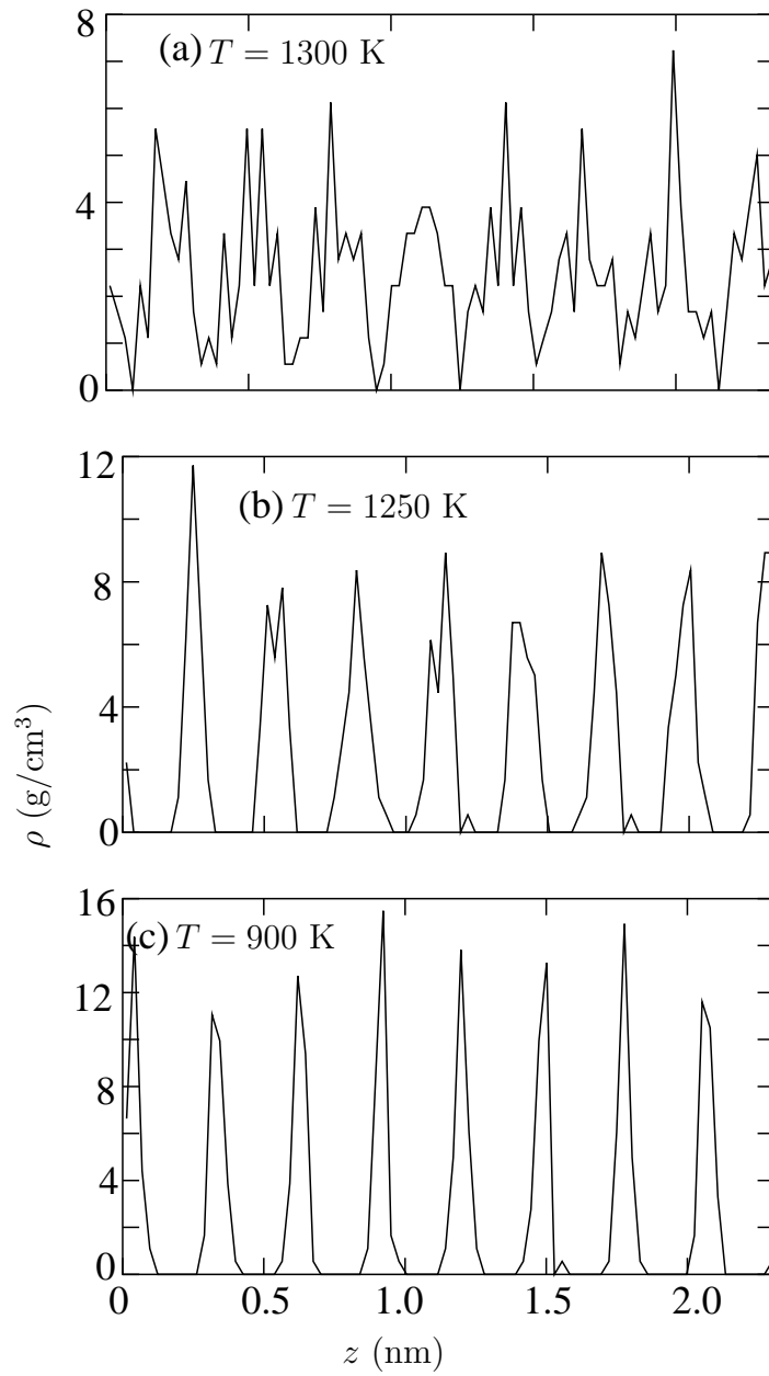
Figure 4: Bulk density profiles along the direction perpendicular to the 111 plane obtained from constant-stress simulations for the EAM Al potential at a pressure of 1 atm and three different temperatures.
