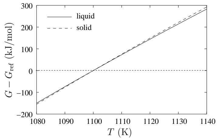
Figure 10: Gibbs free energy (relative to the Gibbs free energy at 1100 K and 1 atm) for both the FCC solid and the liquid phases of EAM Al as a function of temperature.
