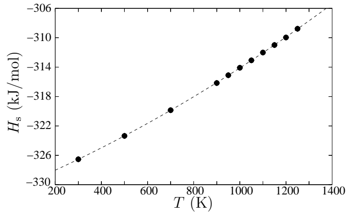
Figure 6: Enthalpy of the bulk fcc solid as a function of temperature for the EAM potential at 1 atm. A quadratic fit is shown by the dashed line with H_s = -330.8 + 0.0130T + 3.644 \times 10^{-6}T^2 .
