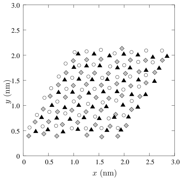
Figure 8: Stacking of the atoms on on three adjacent 111 planes at 1075 K for the solid-slab simulation. Symbols as in Figure 5.
