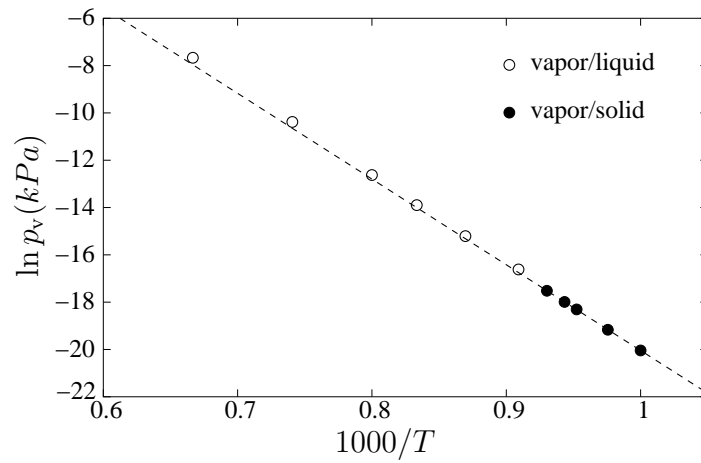
Figure 9: Clausius-Clapeyron plot for the solid-vapor coexistence for the EAM potential represented by the closed circles. The dashed line is the best fit to the sublimation pressure and the open circles are the liquid-vapor data.
